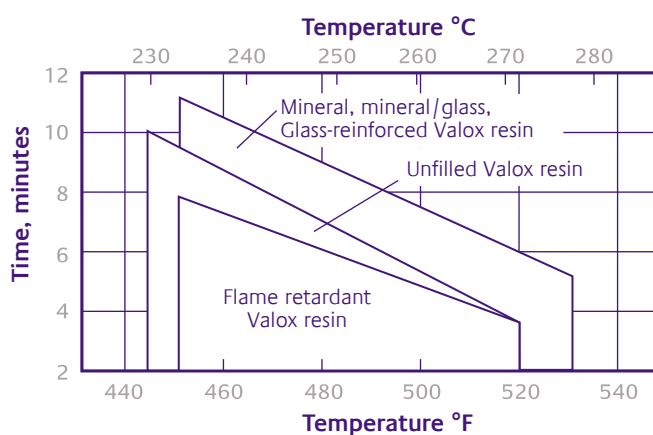
Figure 16.1 – Residence time/temperature area molding diagram
